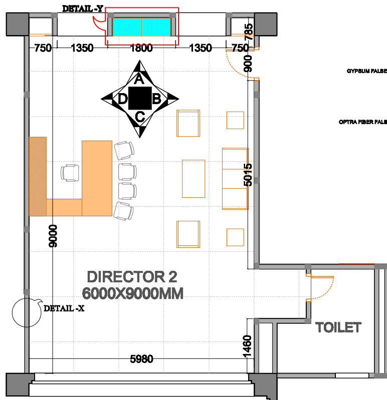
FURNITURE LAYOUT OF THE DIRECTOR'S CABIN- 2
