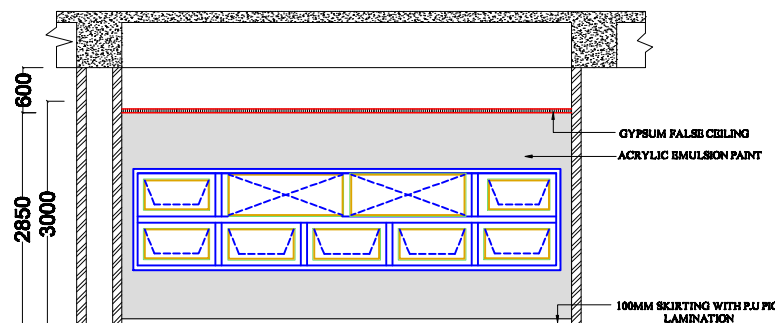
ELEVATION C
