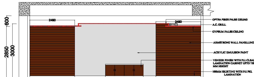
ELEVATION D
