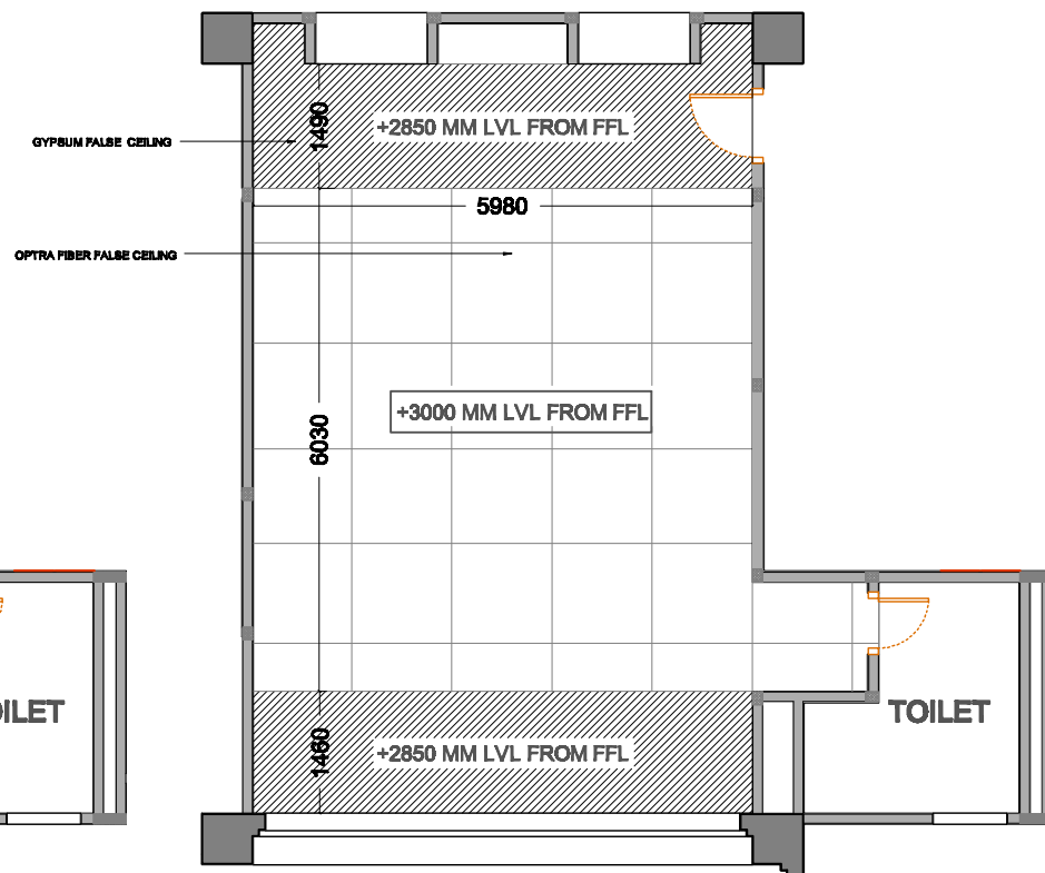
REFLECTED CEILING PLAN LAYOUT
